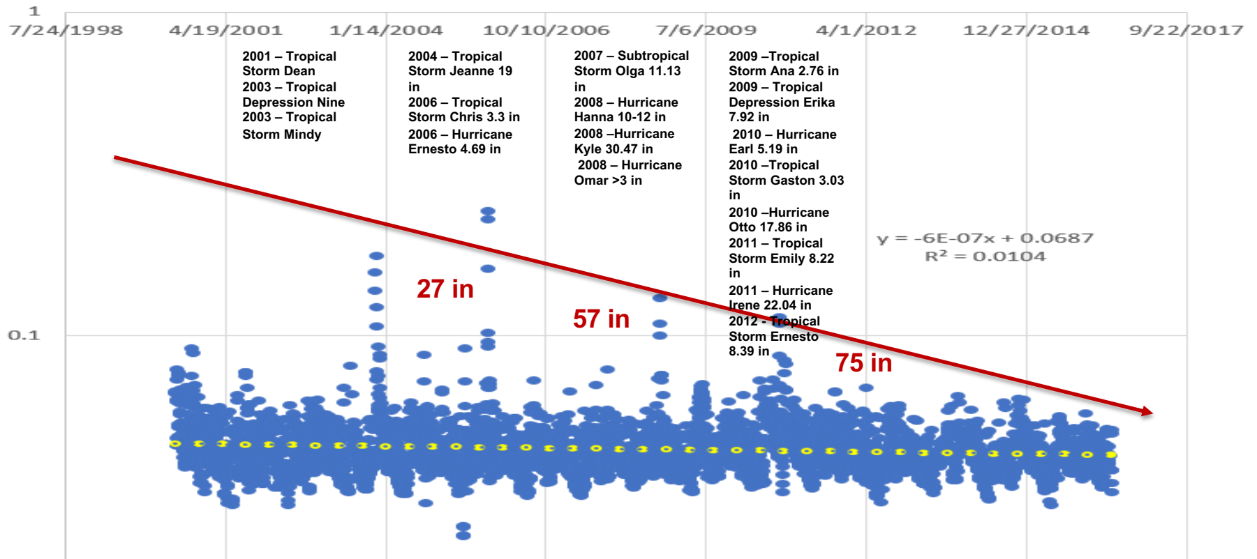
kd_490 m-1, off Guanica Bay
